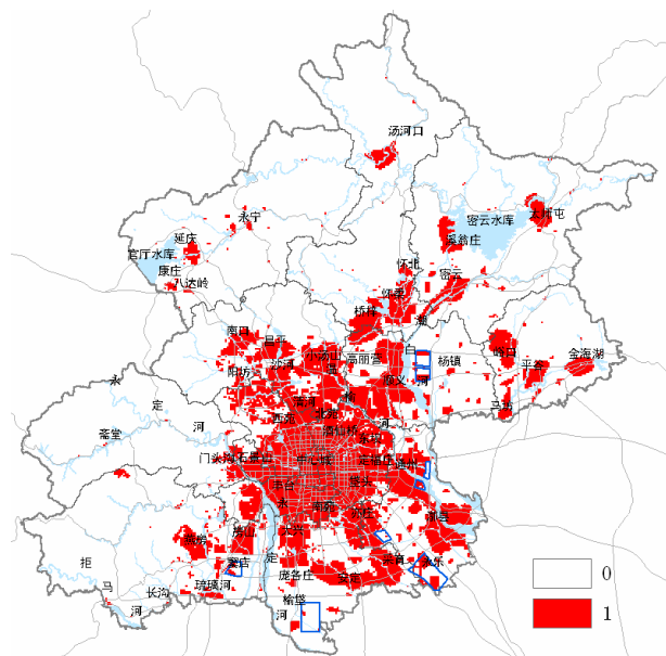
Fig. 7. Simulated urban form of planning controlled scenario
