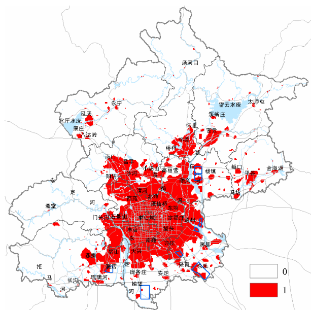
Fig. 6. Simulated urban form of 2001-2006 trend scenario
